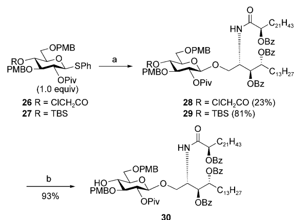
Scheme 5. Synthesis of the Glc-Cer cassette 30 . a) 25 (1 equiv), NIS, TfOH, molecular sieves (4 Å), CH 2 Cl 2 , 0 °C; b) TBAF, THF, 30 °C, 93%. Piv = pivaloyl, TBAF = tetra- n -butylammonium fluoride, TBS = tert -butyldimethylsilyl.
