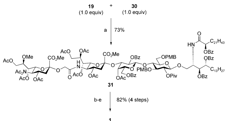
Scheme 6. Final coupling and global deprotection to deliver LLG-3 1 . a) TMSOTf, CH 2 Cl 2 , acid washed molecular sieves (4 Å), 0 °C, 73 %; b) TFA, CH 2 Cl 2 , 0 °C; c) hydrazine acetate, THF, 0 °C; d) LiCl, Py, reflux; e) 0.1 M NaOH (aq.), 0 °C to 45 °C, 82 % (4 steps). TFA = trifluoroacetic acid, TMSOTf = trimethylsilyl trifluoromethanesulfonate.
