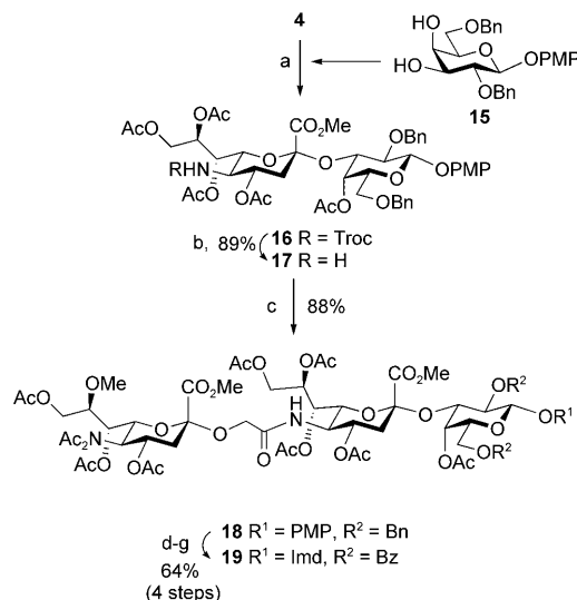
Scheme 3. Synthesis of trisaccharide unit 19 . a) See Ref 8a and 8c for reaction conditions; b) Zn, MeCN/AcOH (4:1), 89%; c) 14 , EDC-HCl, HOBT, NaHCO 3 , MeCN, 88%; d) H 2 , 20% Pd(OH) 2 /C, EtOAc; e) Bz 2 O, DMAP, Py, 40^{\circ}\text{C} , 96% (2 steps); f) CAN, toluene/MeCN/H 2 O (5:6:3), 0^{\circ}\text{C} , 80%; g) CCl 4 CN, DBU, \text{CH}_2\text{Cl}_2 , 0^{\circ}\text{C} , 84%. Bz=benzoyl, CAN=cerium(IV) ammonium nitrate, DBU=1,8-diazabicyclo-[5.4.0]undec-7-ene, EDC=1-ethyl-3-(3-dimethylaminopropyl)carbodiimide, HOBT=1-hydroxybenzotriazole, Imd=trichloroacetimidoyl, PMP= p -methoxyphenyl, Py=pyridine.
