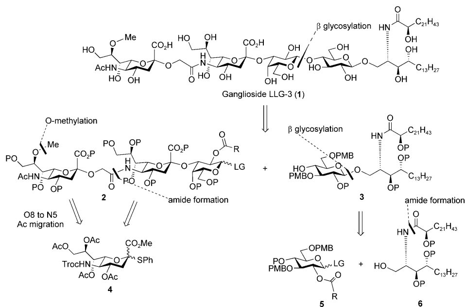
Scheme 1. Retrosynthetic scheme for target molecule 1 . Ac=acetyl, LG=leaving group, P=protecting group, PMB= p -methoxybenzyl, Troc=2,2,2-trichloroethoxycarbonyl.
