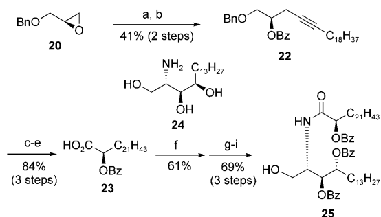
Scheme 4. Synthesis of the ceramide portion 25 . a) 21 , n BuLi, HMPA; b) BzCl, DMAP, Py, 41 % (2 steps); c) H 2 , 10% Pd(OH) 2 /C, EtOAc, RT; d) DMP, NaHCO 3 , CH 2 Cl 2 , RT; e) NaClO 2 , NaH 2 PO 4 , 2-methyl-2-butene, THF/ t BuOH/H 2 O (4:5:1), RT, 84 % (3 steps); f) 24 , EDC·HCl, HOBT, CH 2 Cl 2 , 61 %; g) TrCl, Py, 50 °C; h) BzCl, DMAP, Py, 50 °C, 78 % (2 steps); i) H 2 , 10% Pd(OH) 2 /C, 88 %. DMP = Dess–Martin periodinane, HMPA = hexamethylphosphoric acid triamide, Tr = triphenylmethyl.
